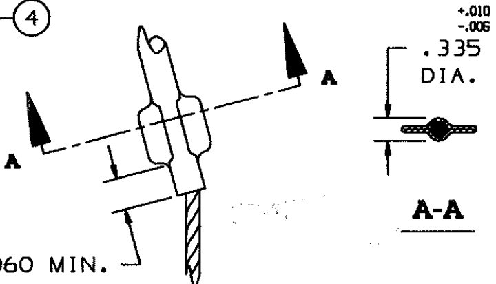
CRIMP DETAIL 2 PL.
