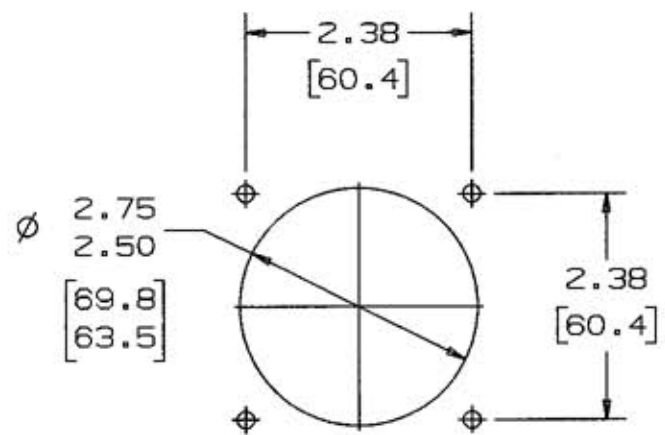
CUTOUT OPENING
