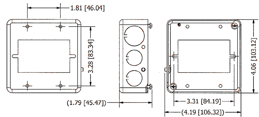
METAL COVER
