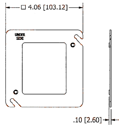
METAL COVER
