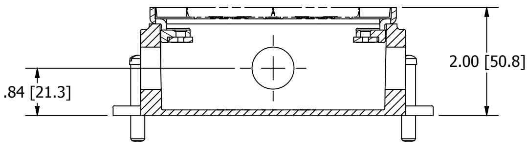
SECTION A-A THROUGH FLOOR BOX
