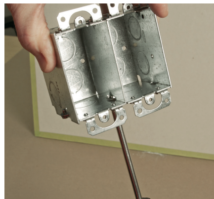
Step 4. Lock partition into position by tightening screws.
