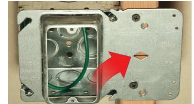
Center window for accurate positioning
