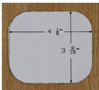
Cut opening Template provided
