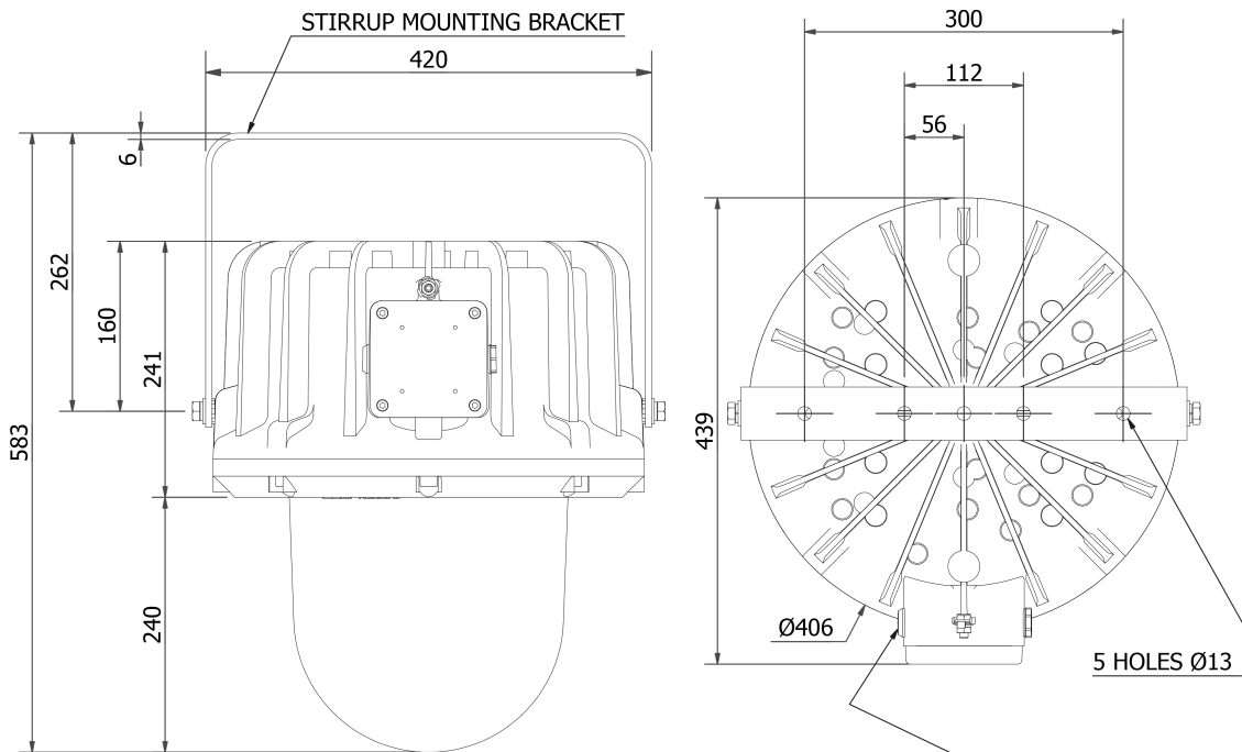
CABLE ENTRY - TWO M20 ENTRIES IN TERMINAL BOX SUPPLIED WITH ONE OFF Ex CERTIFIED BLANKING PLUGS & ONE OFF TRAVELLING PLUG AS STANDARD.
