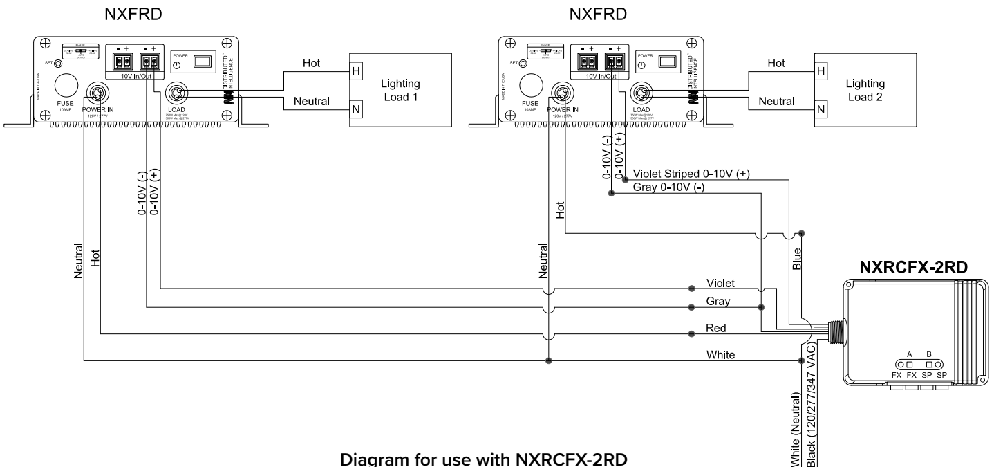
Diagram for use with NXRCFX-2RD
