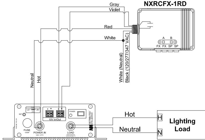
Diagram for use with NXRCX Room Controller
