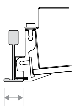
(NG) Narrow Face Grid
