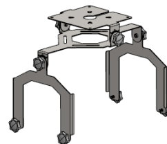
Antenna Retrofit Mount
