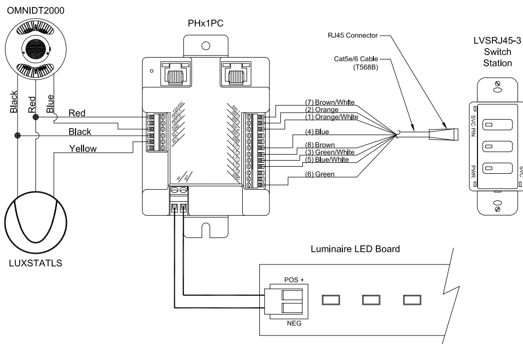
PowerHUBB Master Node with Occupancy Sensor, Daylight Sensor and Low Voltage, 3 Button, RJ45 Enabled Switch Station
