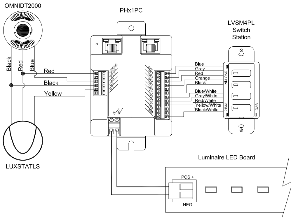
PowerHUBB Master Node with Occupancy Sensor, Daylight Sensor and Low Voltage 4 Button Switch Station
