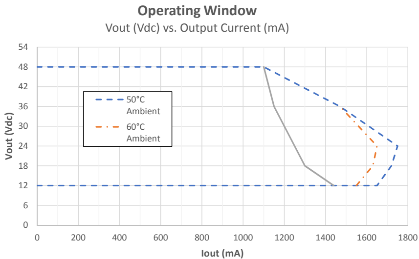
Maximum Output Current vs Load Voltage Fig. 3
