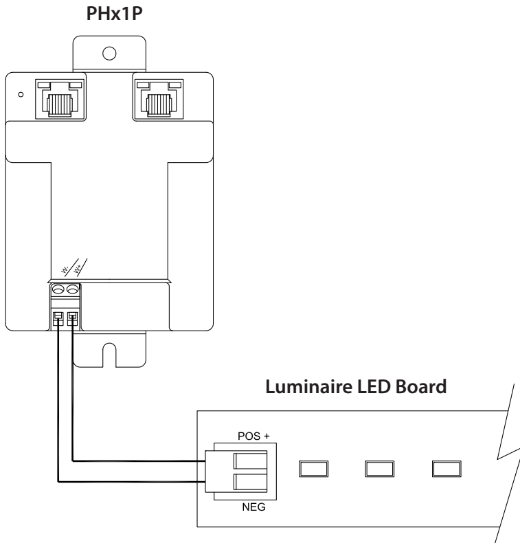
PowerHUBB Master Node connected to LED Board
