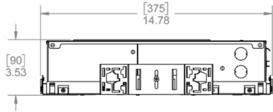
NOR-2.5S Deep Housing Side View
