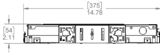
NOR-2.5S Shallow Housing Side View
