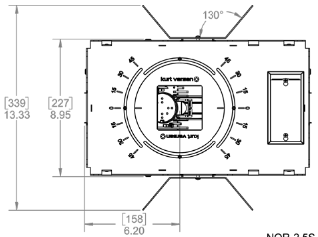
NOR-2.5S ACCENT TRIM WALL WASH TRIM
