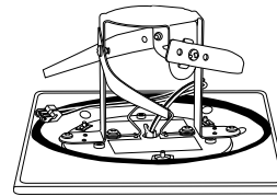
Recessed Adapter
