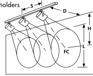
Figure 2 Multiple lampholders
