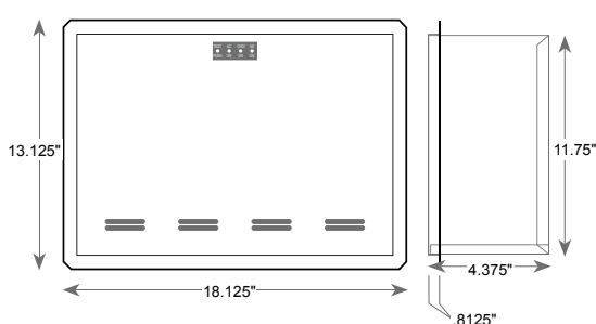
LG125R Recessed Wall Mount Model
