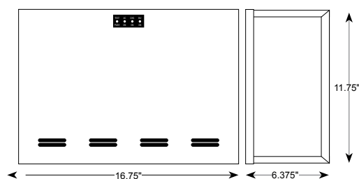
LG250S Wall Mount Surface Model
