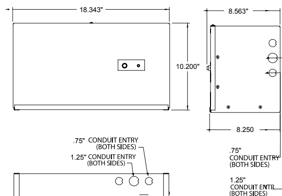
LG2SI Wall Mount Surface Model
