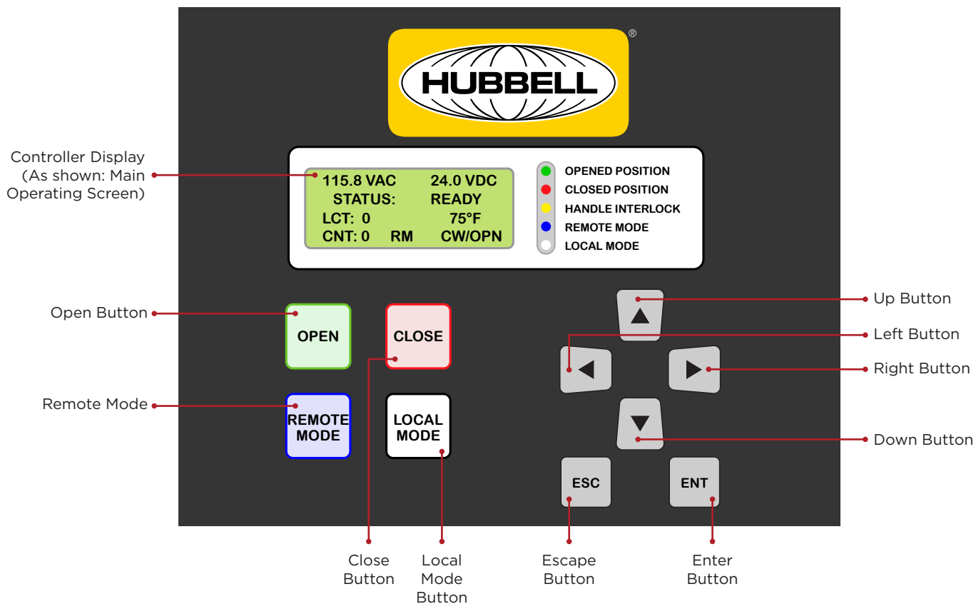
Figure 1. FlexMO motor operator
