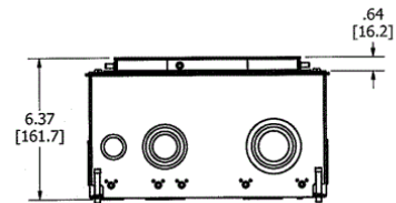
END VIEW
