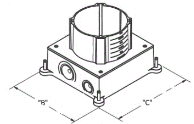
FLOOR BOX WITH COVER ASSEMBLY INSTALLED AT MAXIMUM HEIGHT
