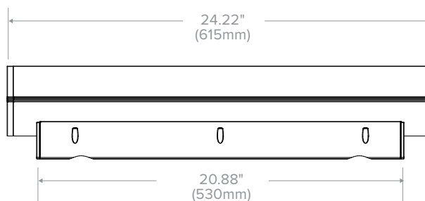
2 FT Fixture
