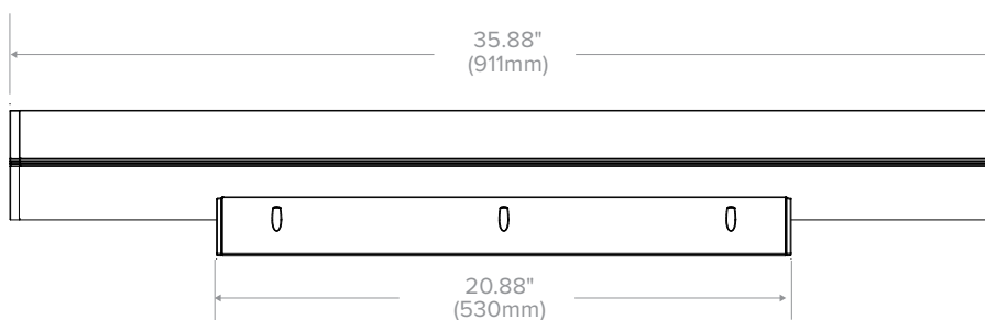
3 FT Fixture
