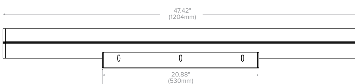
4 FT Fixture
