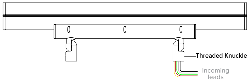
Right Mounting
