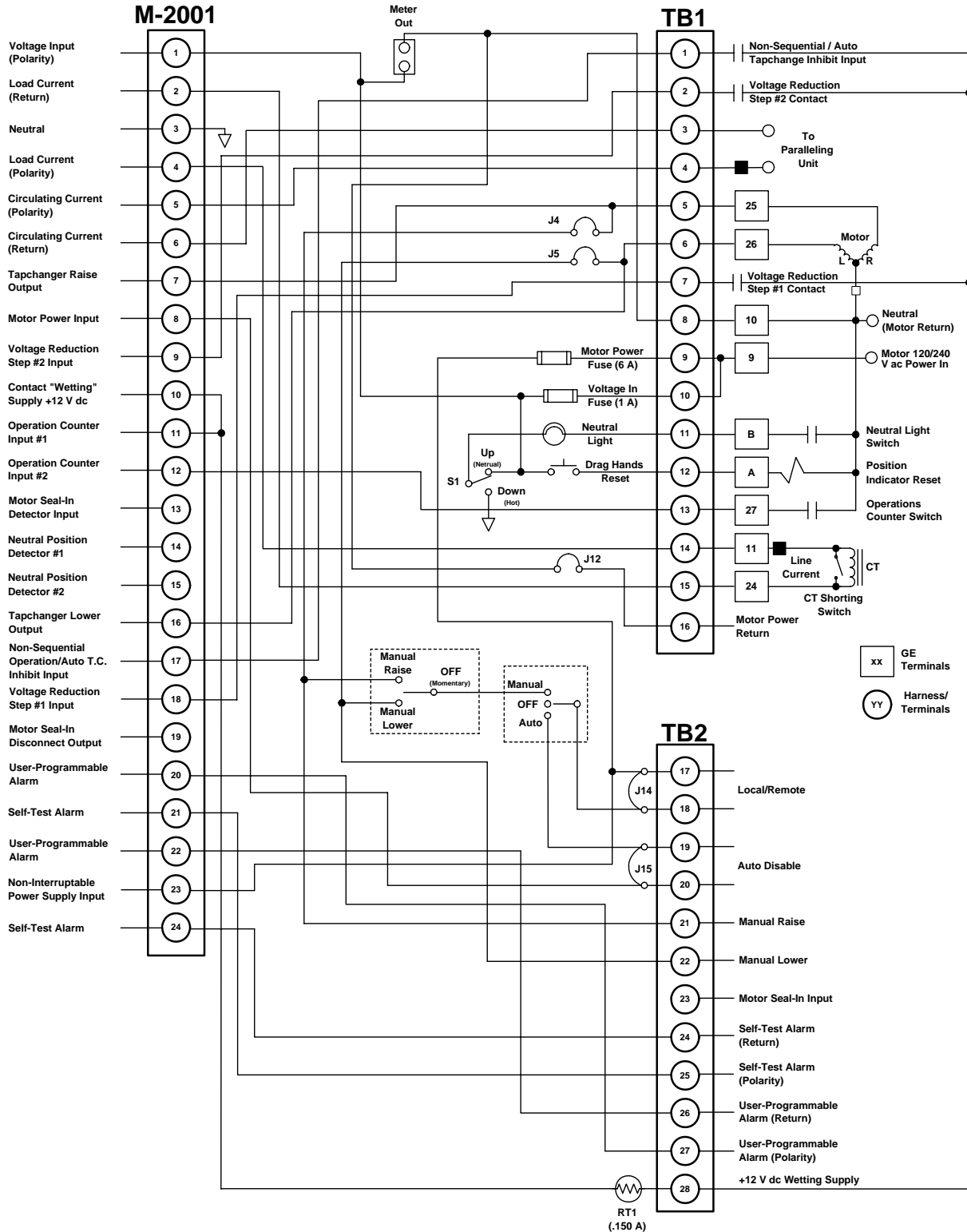
Figure 1 M-2001 (Comprehensive and BASE-T) and M-2264B Panel Typical Connections
