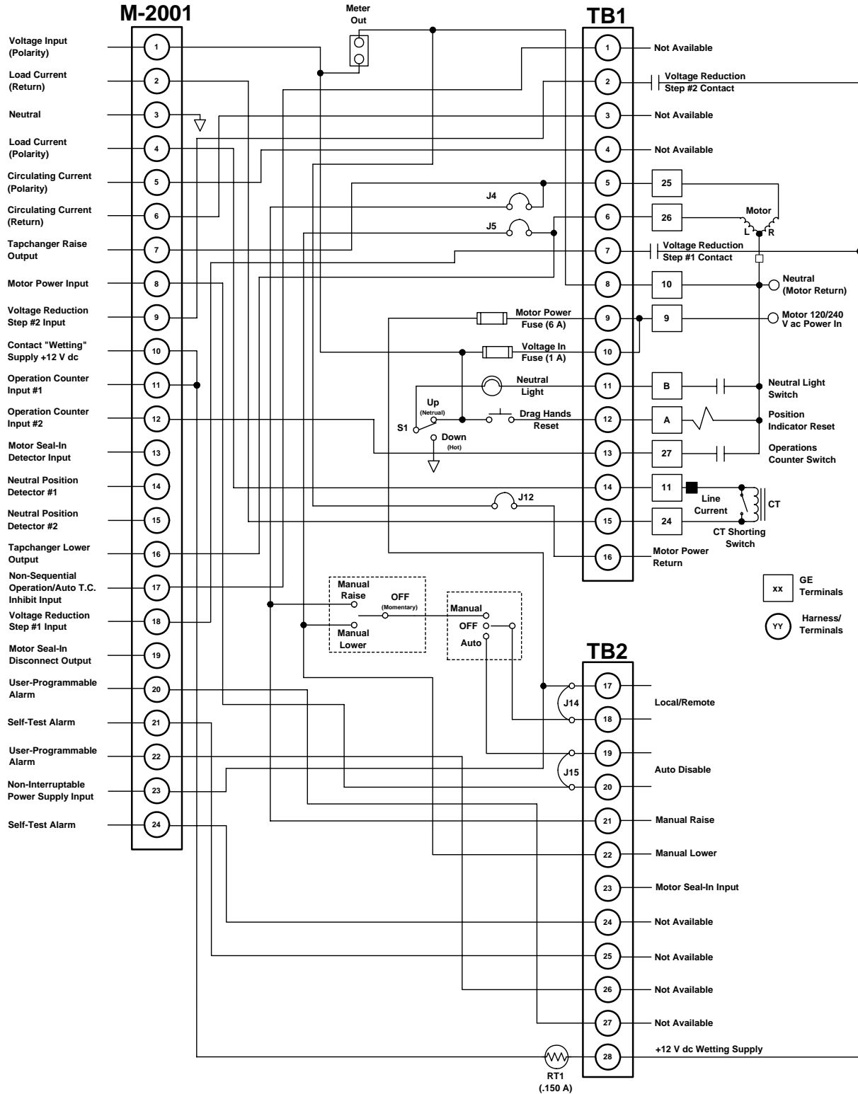
Figure 2 M-2001 (BASE-R) version and M-2264B Panel Typical Connections
