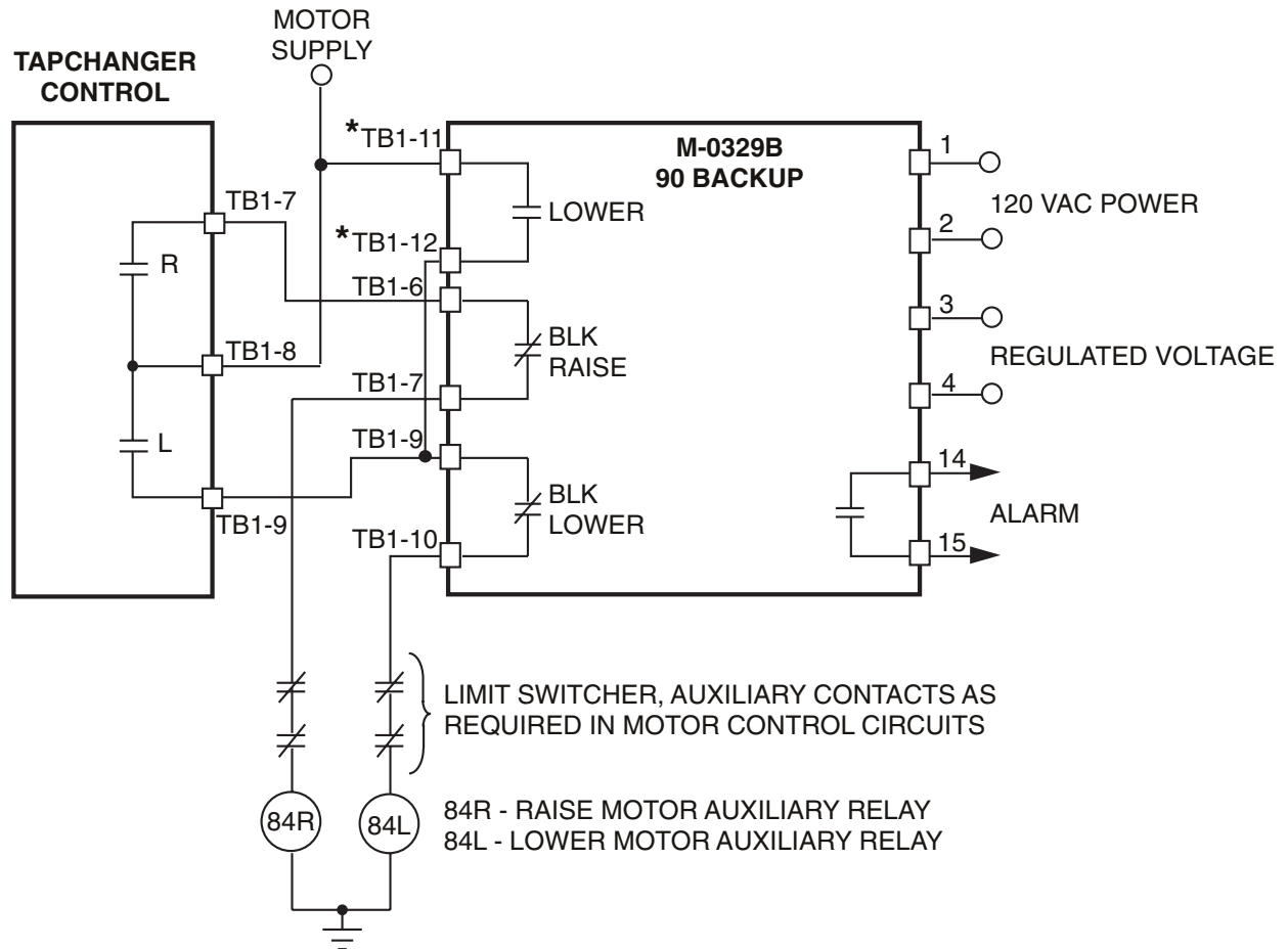
Figure 5 Tapchanger Control and LTC Backup Control Interconnections
