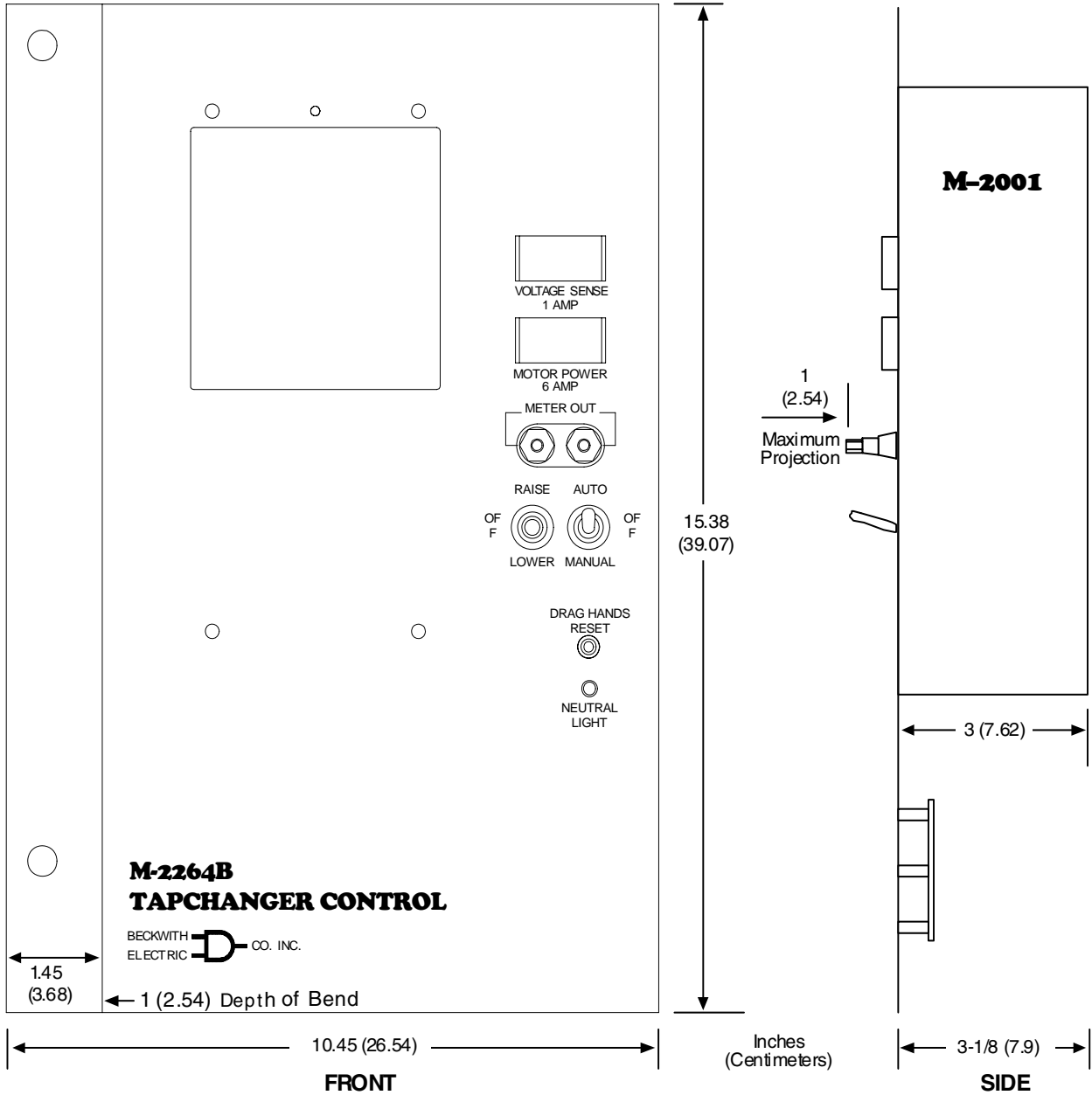
Figure 6 Outline Dimensions
