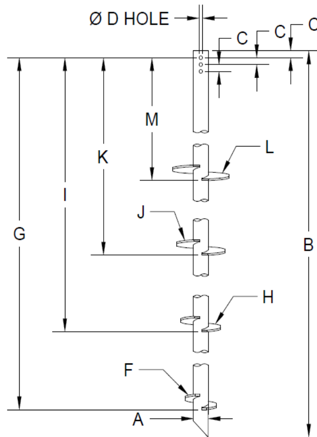
FIGURE 1B—RS2875.203, RS2875.276 & RS3500 LEAD SECTIONS
