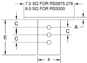
FIGURE 7B—NEW CONSTRUCTION PILE CAP FOR RS2875.203 & 276 & RS3500
