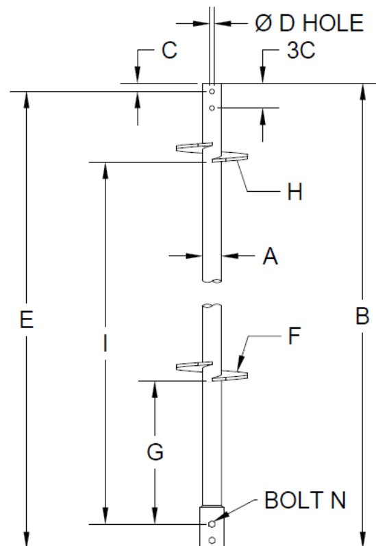
FIGURE 1B—RS2875.203, RS2875.276 & RS3500 LEAD SECTIONS
