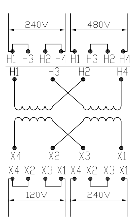
CONNECTION DIAGRAM
