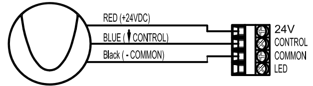
DAYLIGHT SENSOR
