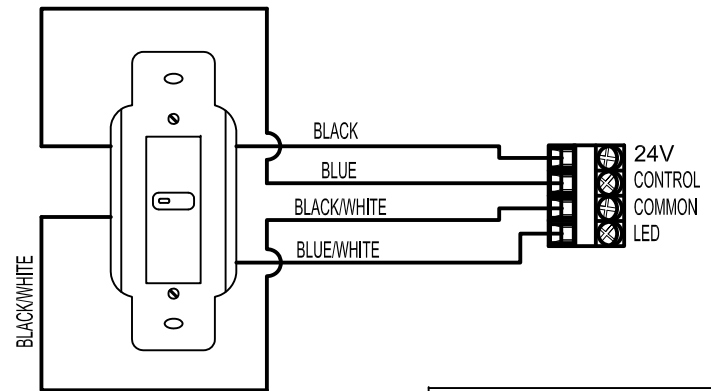
LVSL1PLSwitch Station
