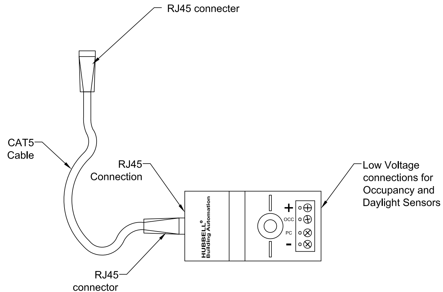
RJ45ADAPTER (Top View)
